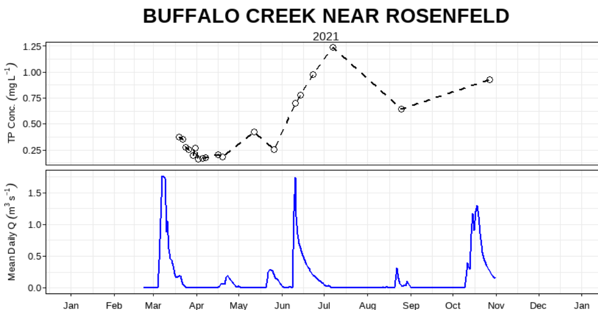
Figure 14: Mean daily discharge (m 3 s -1 ) and total phosphorus concentration (mg L -1 ) over the 2021 sampling season at Buffalo Creek near Rosenfeld (05OC019).
