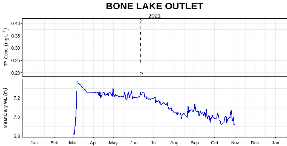
Figure 24: Water depth and total phosphorus concentration at Bone Lake Outlet (05OA019).
