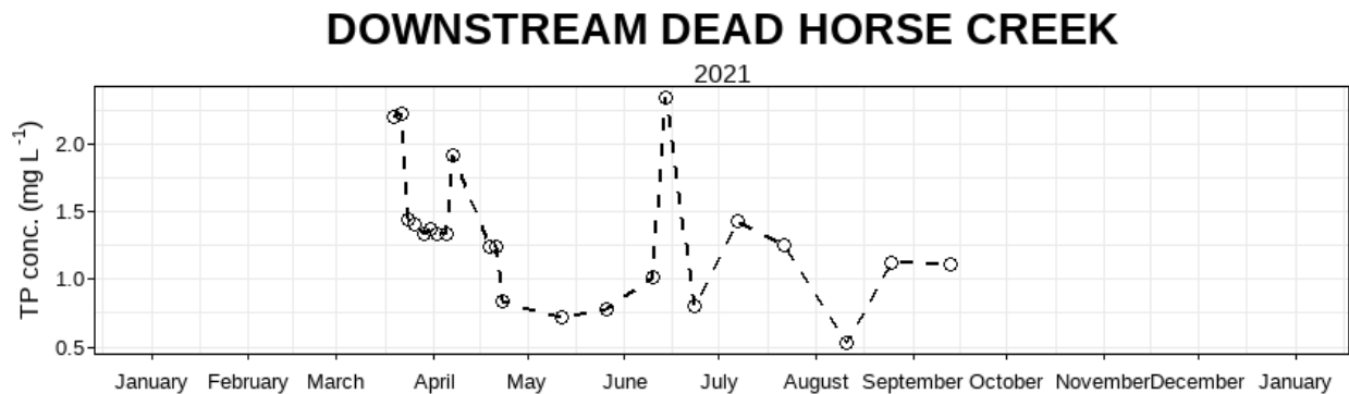
Figure 22: Total phosphorus concentration at Downstream Deadhorse Creek in 2021.
