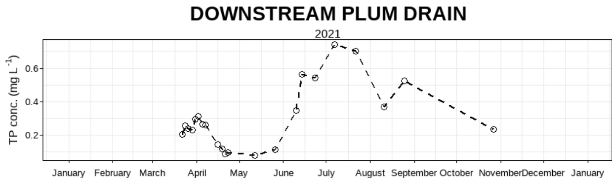
Figure 23: Total phosphorus concentration at Downstream Plum Drain in 2021.
