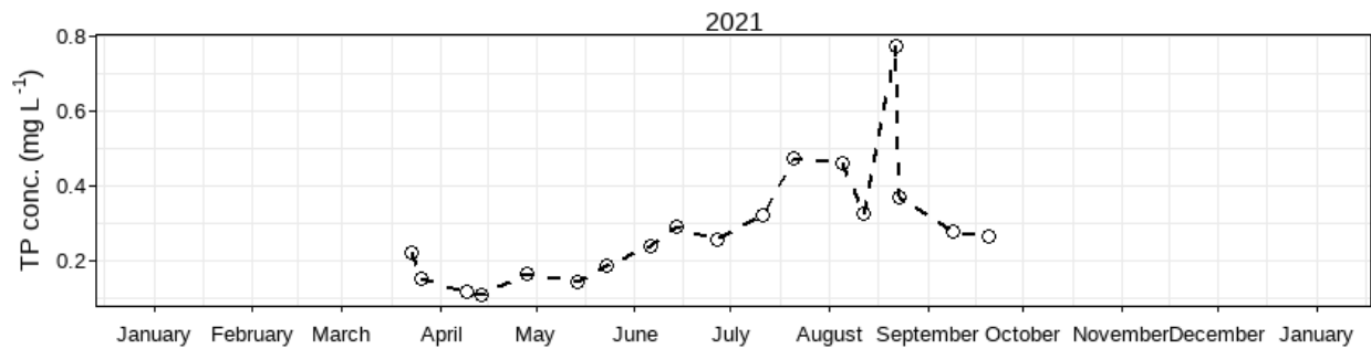
Figure 8: Total phosphorus concentration (mg L -1 ) over the 2021 sampling season at Seine River near Park Lagimodière-Gaboury (05NG021).
