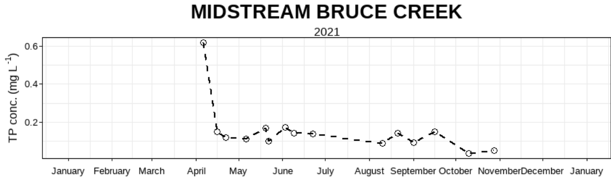
Figure 10: Total phosphorus concentration (mg L -1 ) over the 2021 sampling season at Midstream Bruce Creek.
