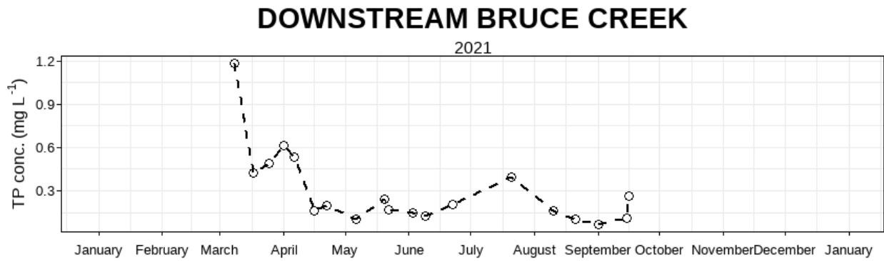
Figure 11: Total phosphorus concentration (mg L -1 ) over the 2021 sampling season at Downstream Bruce Creek.
