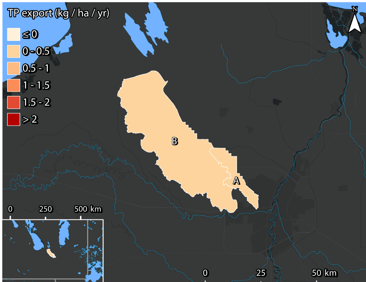
Figure 3: 2021 LWCBMN TP Export Hotspots in City of Winnipeg. Letters correspond to sites listed in Table 2.
