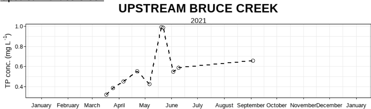
Figure 9: Total phosphorus concentration (mg L -1 ) over the 2021 sampling season at Upstream Bruce Creek.
