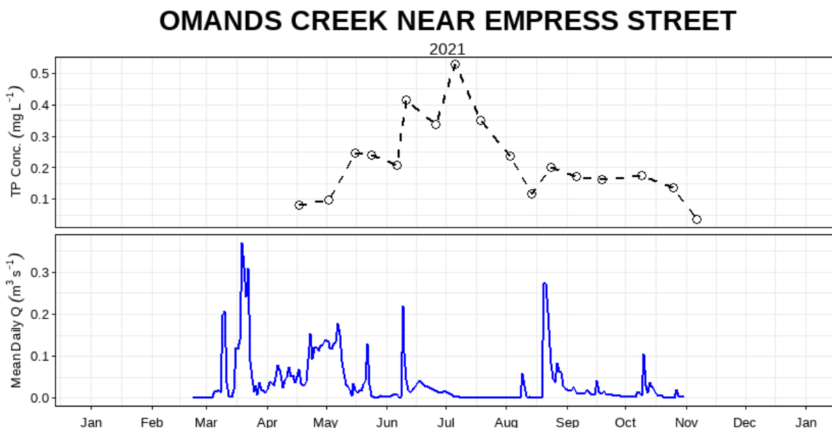
Figure 4: Mean daily discharge (m 3 s -1 ) and total phosphorus concentration (mg L -1 ) over the 2021 sampling season at Omand’s Creek near Empress Street (05MJ013).
