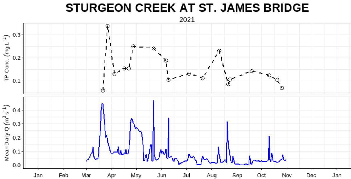
Figure 6: Mean daily discharge (m 3 s -1 ) and total phosphorus concentration (mg L -1 ) over the 2021 sampling season at Sturgeon Creek at St. James Bridge (05MJ004).
