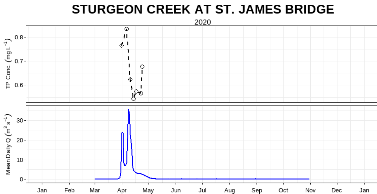
Figure 6: Mean daily discharge (m 3 s -1 ) and total phosphorus concentration (mg L -1 ) over the 2020 sampling season at Sturgeon Creek at St. James Bridge (05MJ004).
