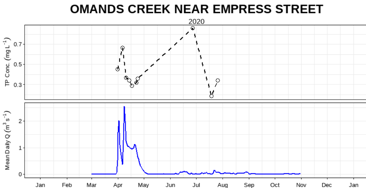
Figure 4: Mean daily discharge (m 3 s -1 ) and total phosphorus concentration (mg L -1 ) over the 2020 sampling season at Omand’s Creek near Empress Street (05MJ013).
