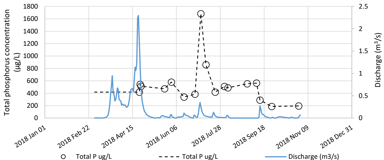
Figure 7. Discharge and total phosphorus concentration over the 2018 sampling season at Grassmere Creek Drain near Middlechurch (Water Survey of Canada Station 05OJ017).
