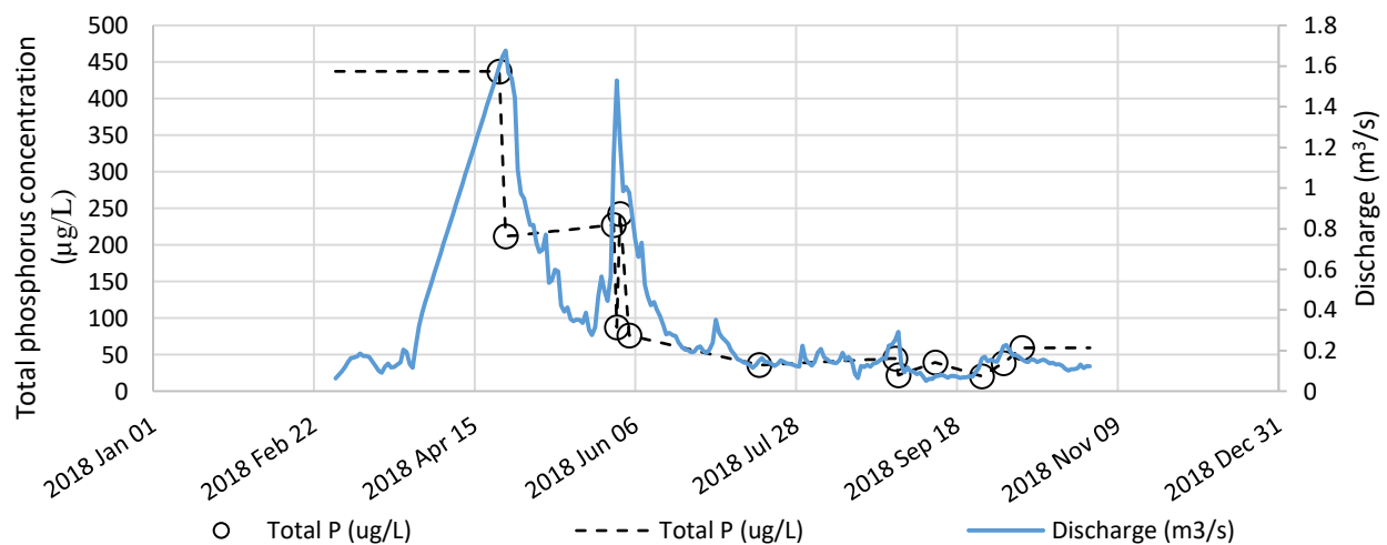
Figure 4. Discharge and total phosphorus concentration over the 2018 sampling season at Fisher River near Fisherton (Water Survey of Canada Station 05SD005).
