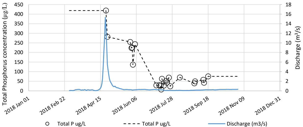
Figure 5. Discharge and total phosphorus concentration over the 2018 sampling season at Icelandic River near Riverton (Water Survey of Canada Station 05SC002).
