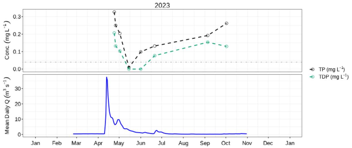
Figure 6: Mean daily discharge (blue) with TP (black) & TDP concentration (green) at Whitemud River near Keys (05LL005).
