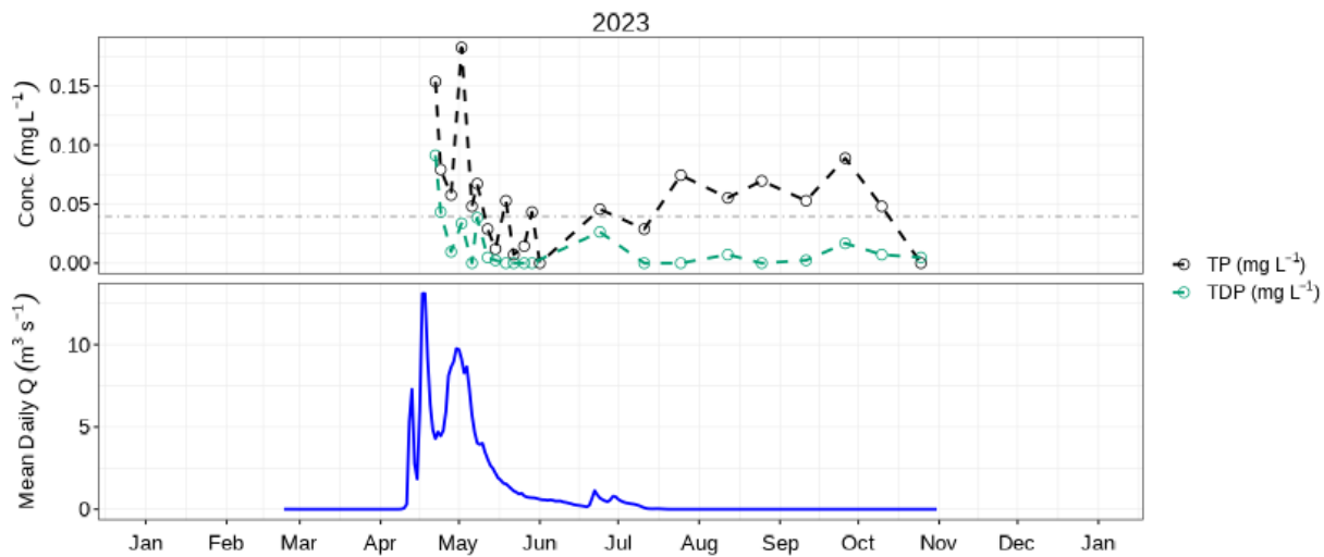
Figure 4: Mean daily discharge (blue) with TP (black) & TDP concentration (green) at Big Grass River near Glenella (05LL015).
