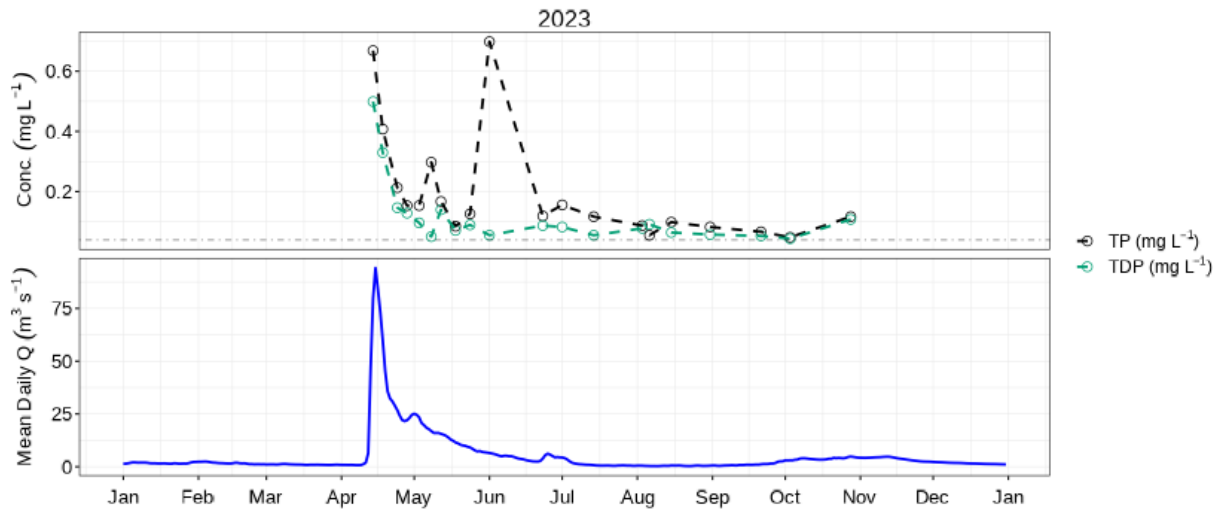
Figure 8: Mean daily discharge (blue) with TP (black) & TDP concentration (green) at Whitemud River near Westbourne (05LL002).
