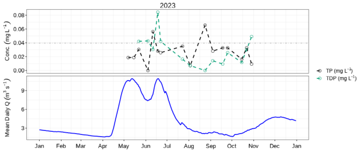
Figure 6: Mean daily discharge (blue) with TP (black) & TDP concentration (green) at Bird River outlet of Bird Lake (05PJ001).
