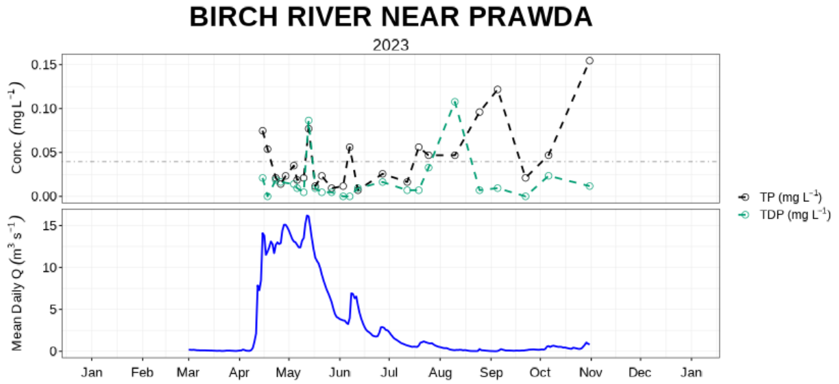
Figure 4: Mean daily discharge (blue) with TP (black) & TDP concentration (green) at Birch River near Prawda (05PH007).
