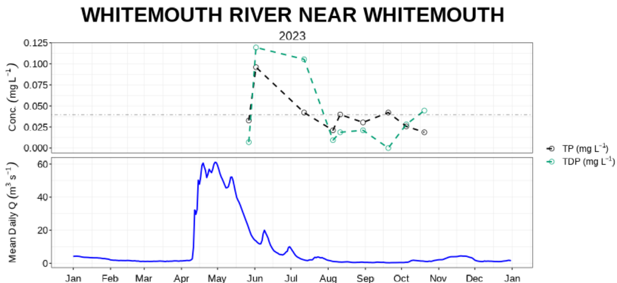
Figure 10: Mean daily discharge (blue) with TP (black) & TDP concentration (green) at Whitemouth River near Whitemouth (05PH003).
