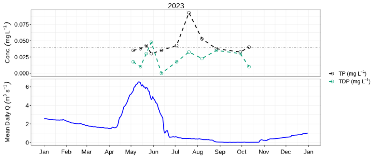
Figure 8: Mean daily discharge (blue) with TP (black) & TDP concentration (green) at Whiteshell River at outlet of Jessica Lake (05PG001).
