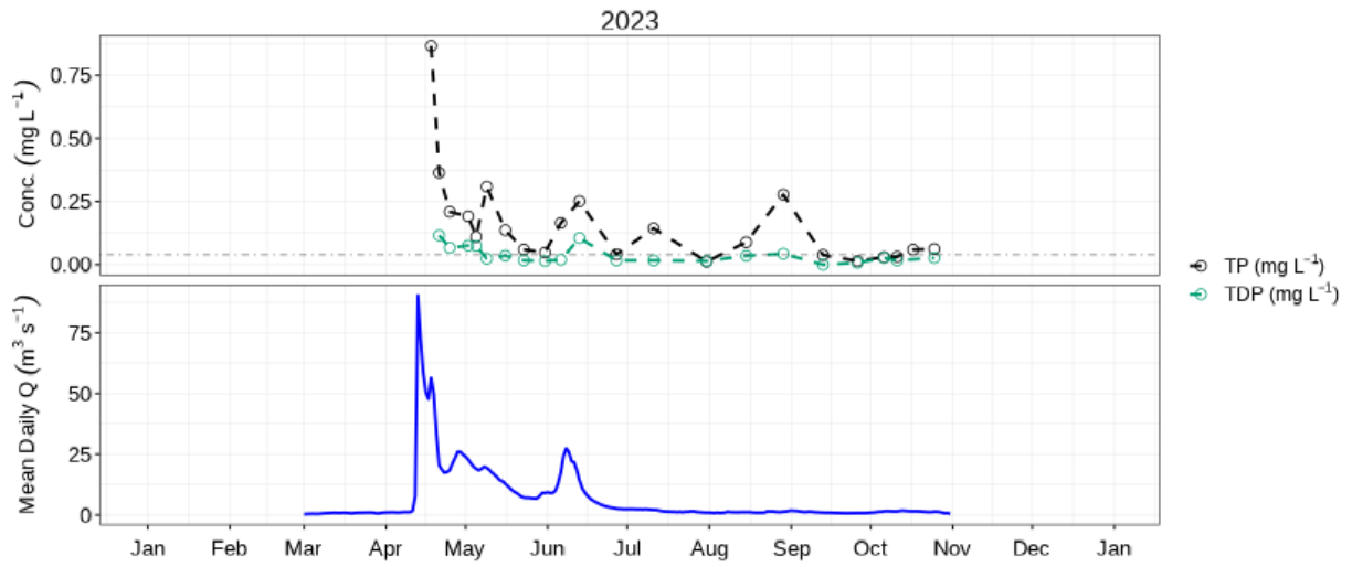
Figure 10: Mean daily discharge (blue) with TP (black) & TDP concentration (green) at Swan River near Minitonas (05LE006).
