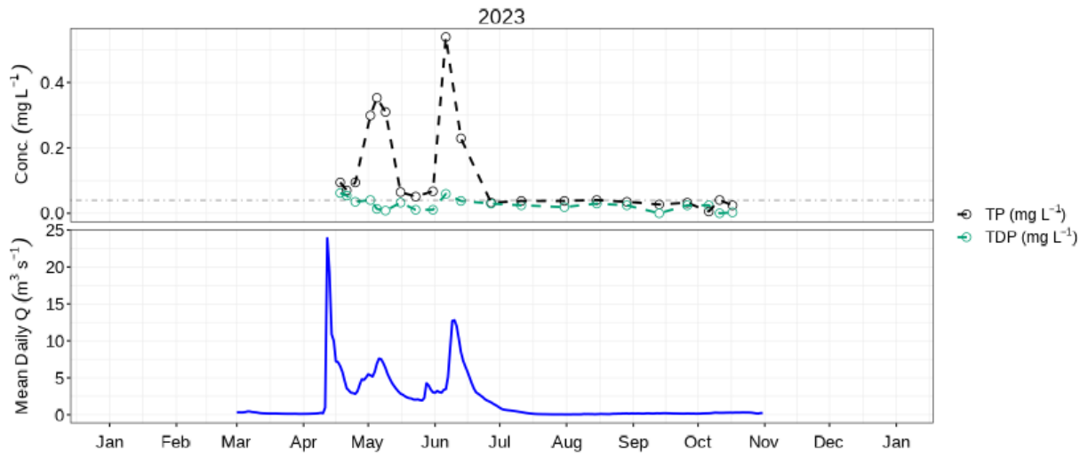
Figure 8: Mean daily discharge (blue) with TP (black) & TDP concentration (green) at Roaring River near Minitonas (05LE005).
