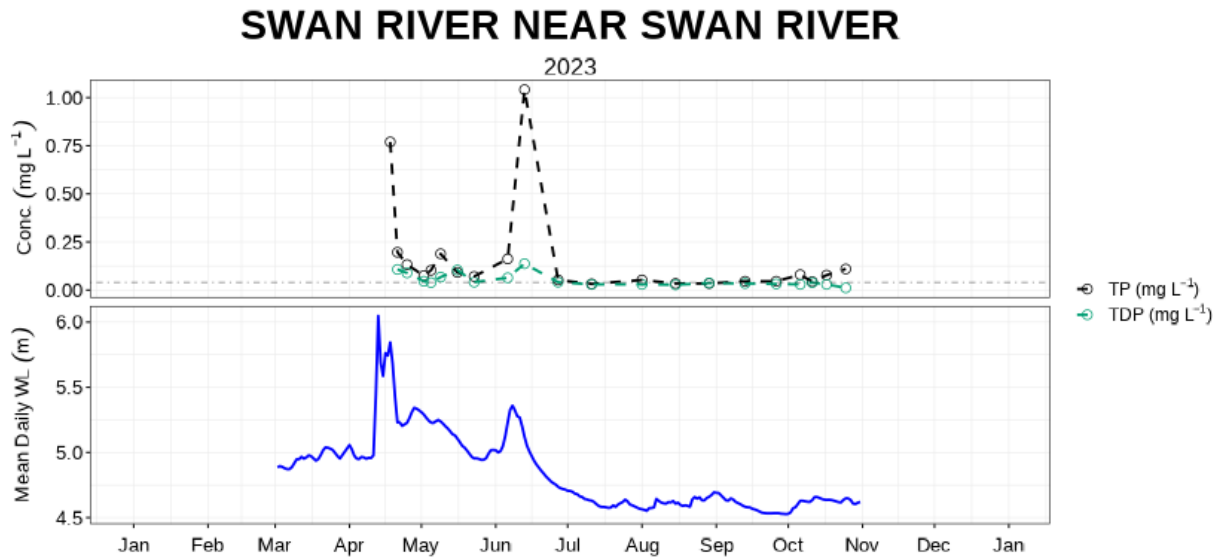
Figure 14: Mean daily water level (blue) with TP (black) & TDP concentration (green) at Swan River near Swan River (05LE001).
