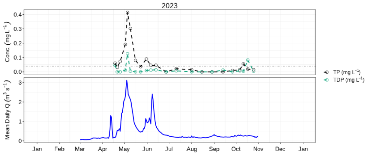
Figure 4: Mean daily discharge (blue) with TP (black) & TDP concentration (green) at Birch River near Birch River (05LE010).
