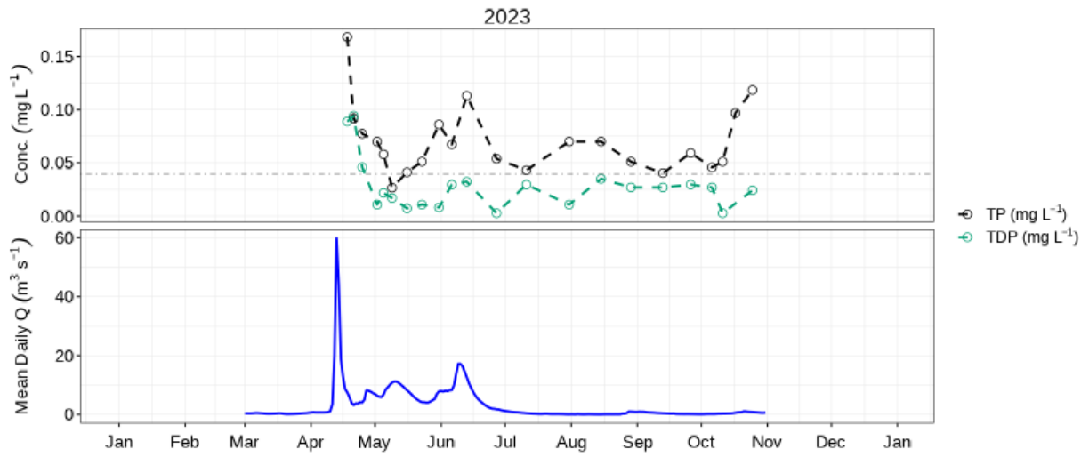
Figure 12: Mean daily discharge (blue) with TP (black) & TDP concentration (green) at Woody River near Bowsman (05LE004).
