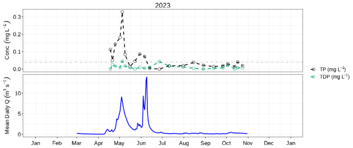
Figure 6: Mean daily discharge (blue) with TP (black) & TDP concentration (green) at North Duck River at Cowan (05LG004).
