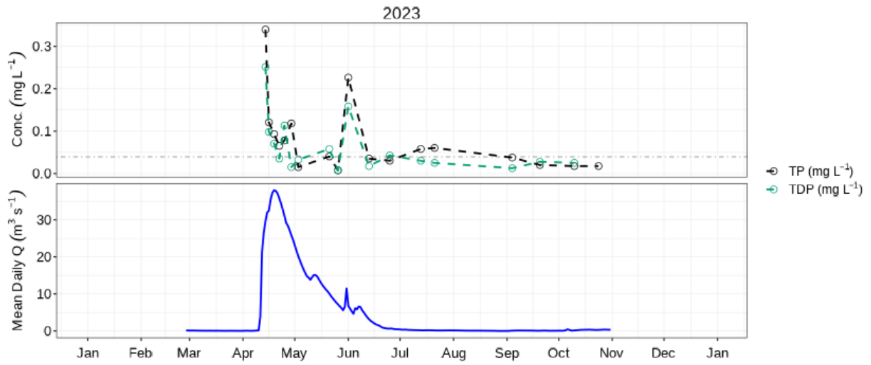
Figure 4: Mean daily discharge (blue) with TP (black) & TDP concentration (green) at Brokenhead River at Beausejour (05SA002).
