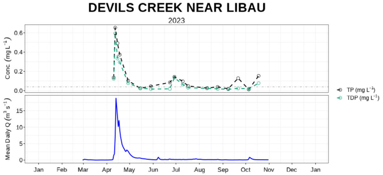
Figure 6: Mean daily discharge (blue) with TP (black) & TDP concentration (green) at Devil's Creek near Libau (05OJ016).
