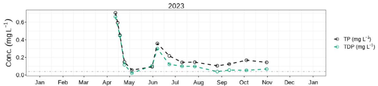
Figure 9: Mean daily discharge (blue) with TP (black) & TDP concentration (green) at Cooks Creek Downstream.
