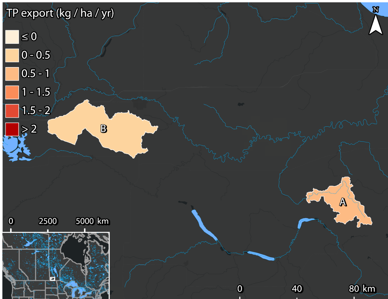
Figure 3: 2023 LWCBMN TP Export Hotspots in Central Assiniboine. Letters correspond to sites listed in Table 2.
