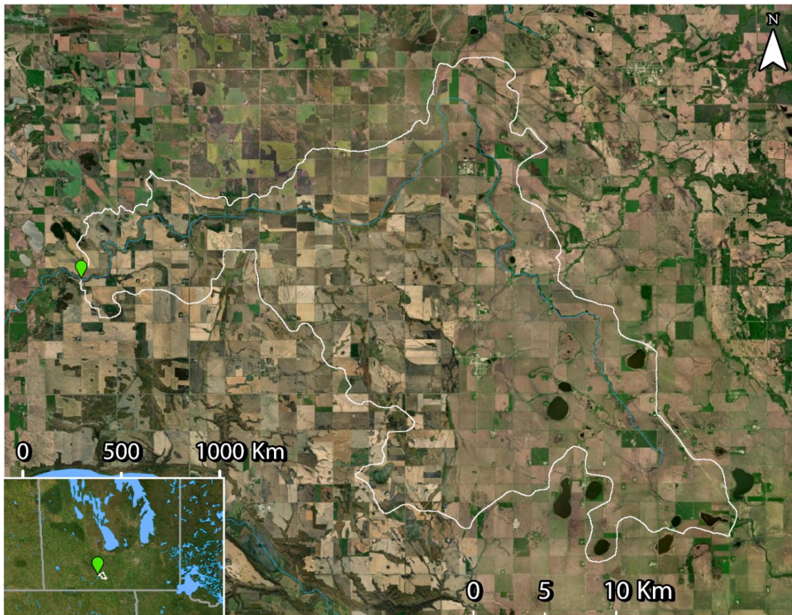
Figure 5: WSC station 05MH008 (green) and drainage area polygon (white - source: WSC). LWCBMN samples directly at the WSC station.
