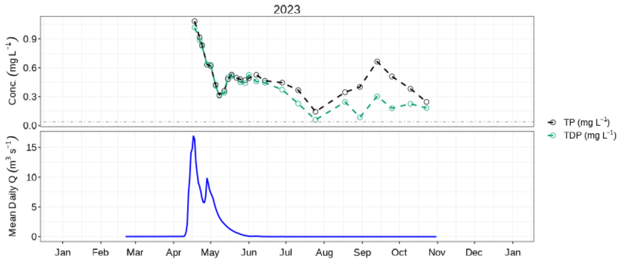
Figure 4: Mean daily discharge (blue) with TP (black) & TDP concentration (green) at Cypress River near Bruxelles (05MH008).
