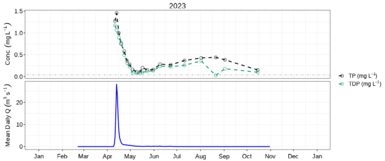
Figure 6: Mean daily discharge (blue) with TP (black) & TDP concentration (green) at Little Souris River near Brandon (05MH006).
