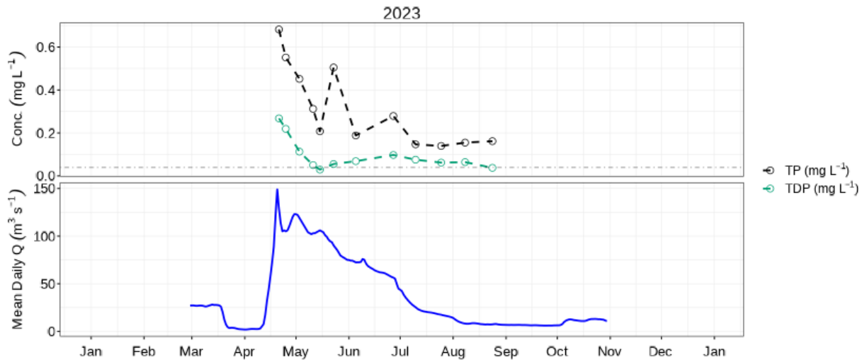
Figure 8: Mean daily discharge (blue) with TP (black) & TDP concentration (green) at Assiniboine River near Miniota (05ME006).
