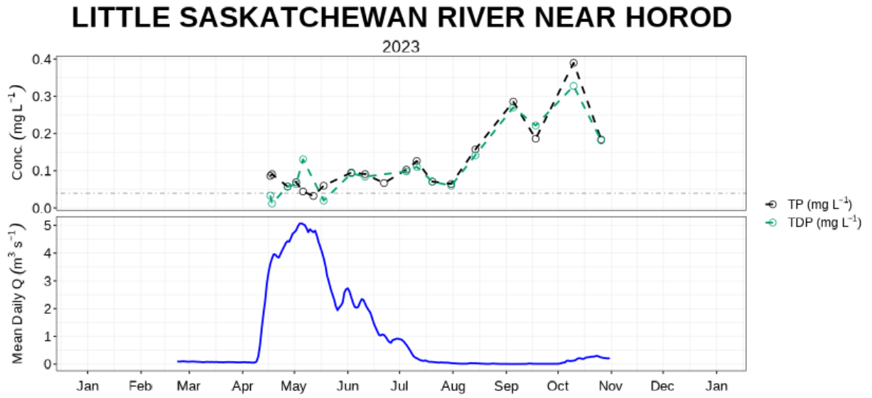
Figure 14: Mean daily discharge (blue) with TP (black) & TDP concentration (green) at Little Saskatchewan River near Horod (05MF024).
