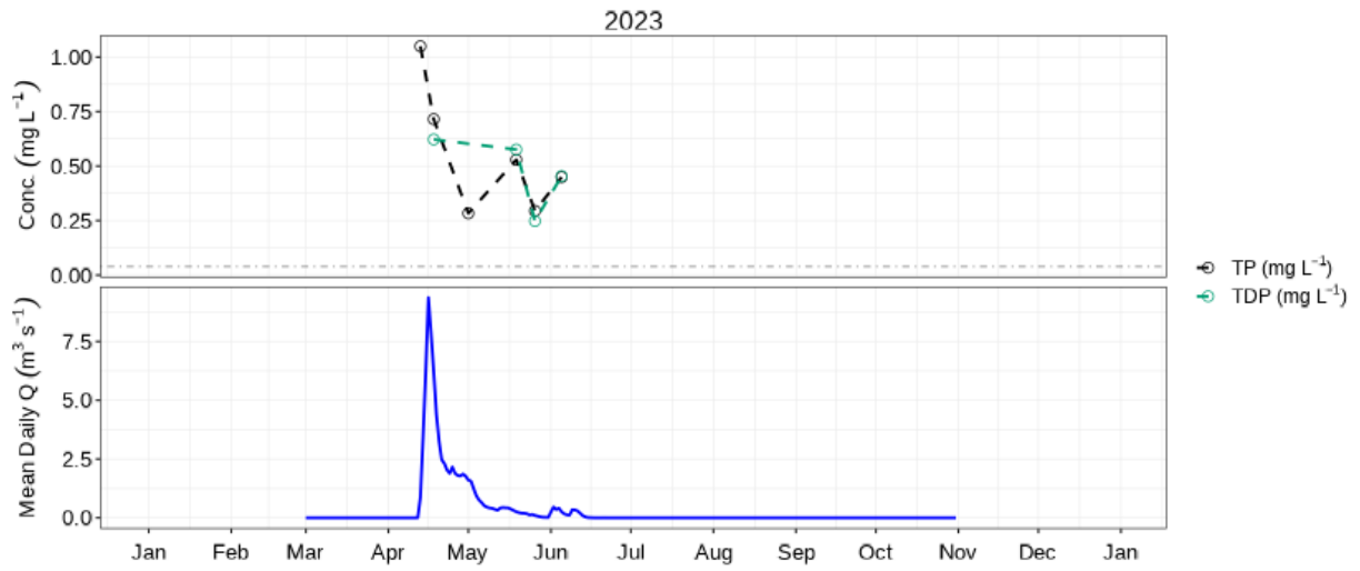
Figure 12: Mean daily discharge (blue) with TP (black) & TDP concentration (green) at Gopher Creek near Virden (05MG003).
