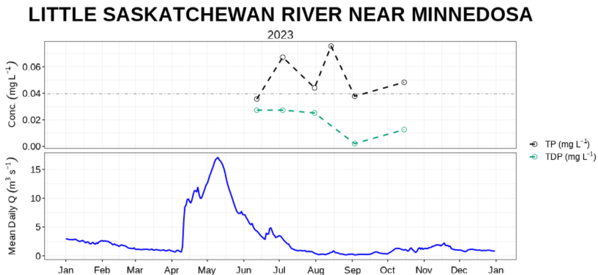
Figure 20: Mean daily discharge (blue) with TP (black) & TDP concentration (green) at Little Saskatchewan River near Minnedosa (05MF001).
