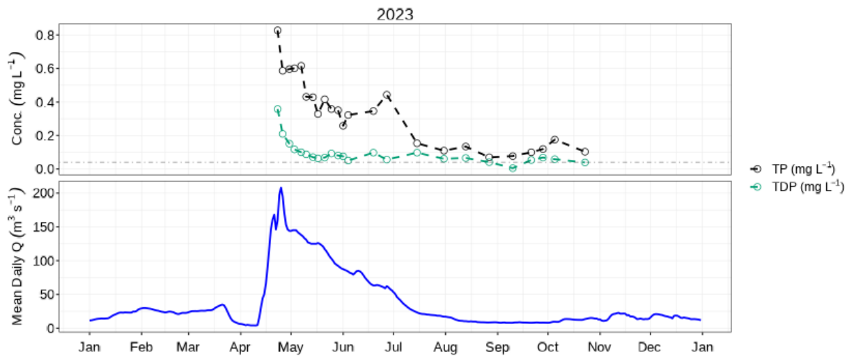
Figure 6: Mean daily discharge (blue) with TP (black) & TDP concentration (green) at Assiniboine River near Brandon (05MH001).
