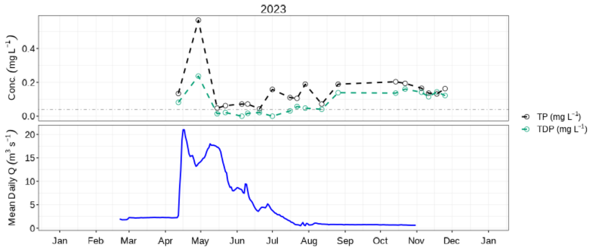
Figure 16: Mean daily discharge (blue) with TP (black) & TDP concentration (green) at Little Saskatchewan River near Rivers (05MF018).
