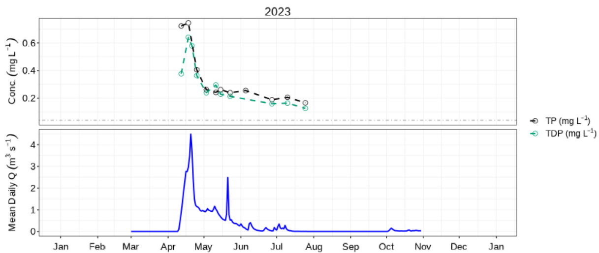
Figure 4: Mean daily discharge (blue) with TP (black) & TDP concentration (green) at Arrow River near Arrow River (05MG001).
