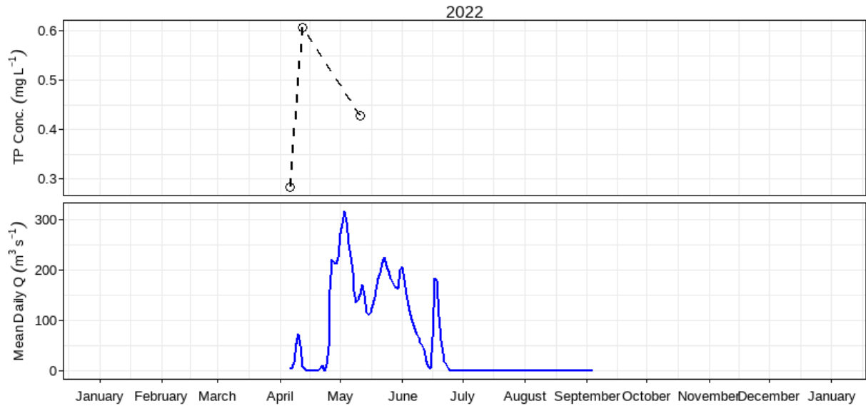
Figure 29: Mean daily discharge (m 3 s -1 ) and total phosphorus concentration (mg L -1 ) over the 2022 sampling season at Portage Diversion near Portage La Prairie (05LL019).
