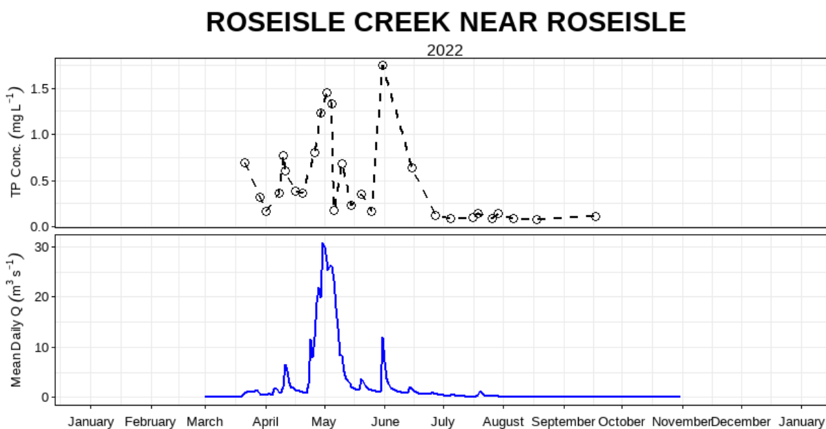
Figure 12: Mean daily discharge (m 3 s -1 ) and total phosphorus concentration (mg L -1 ) over the 2022 sampling season at Roseisle Creek near Roseisle (05OF009).
