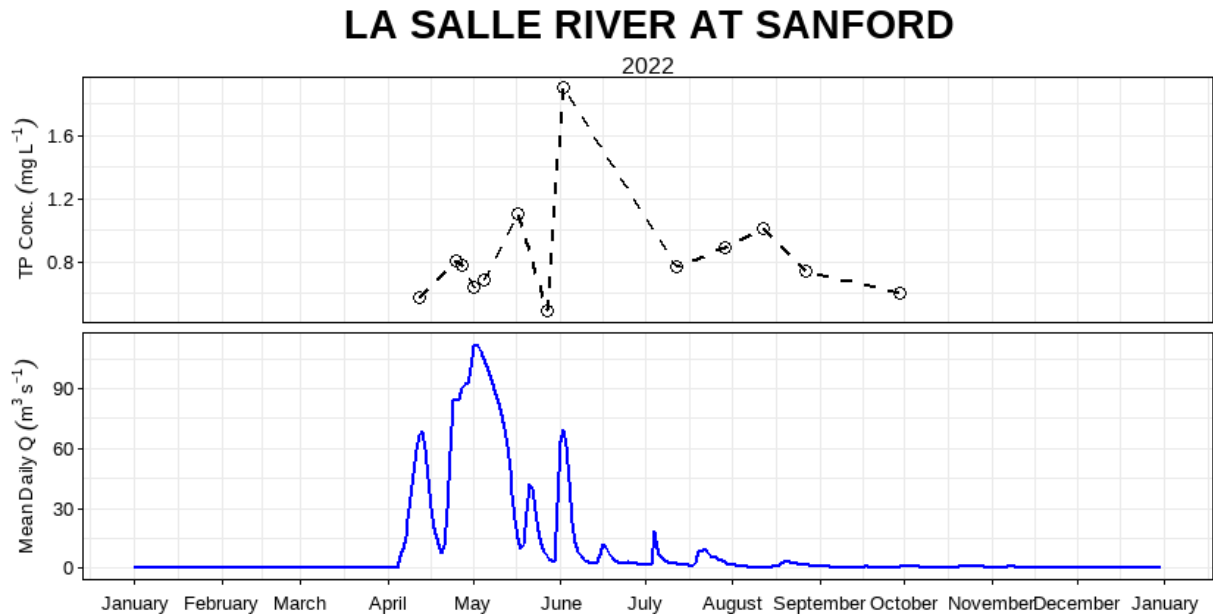
Figure 26: Mean daily discharge (m 3 s -1 ) and total phosphorus concentration (mg L -1 ) over the 2022 sampling season at La Salle River at Sanford (05OG001).
