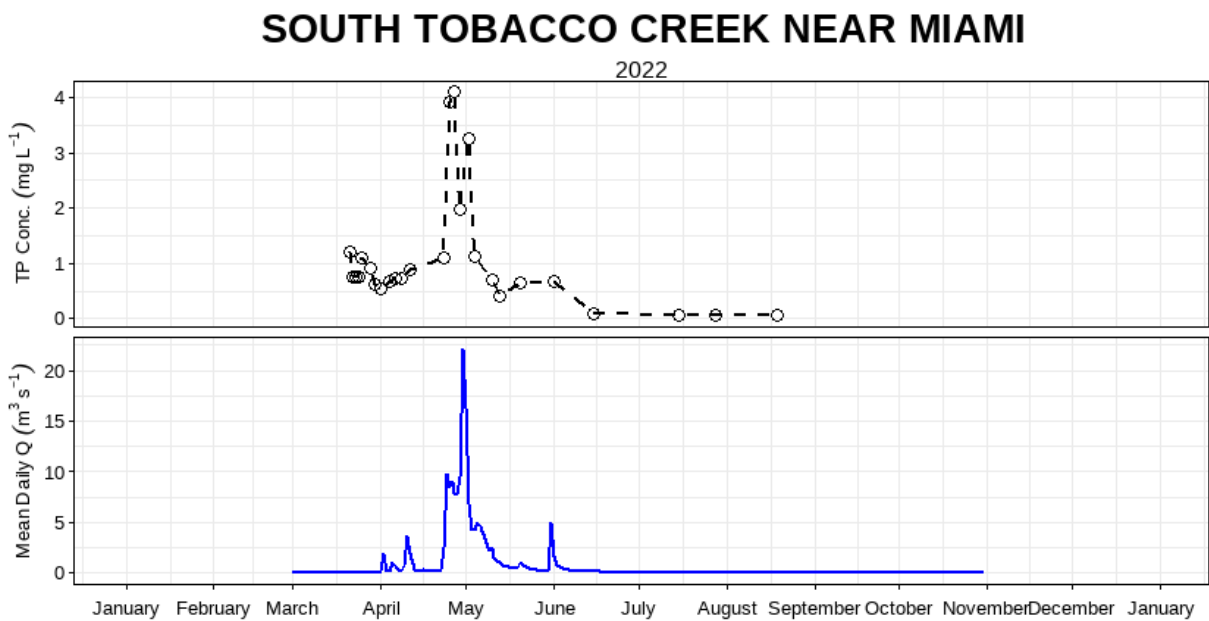
Figure 14: Mean daily discharge (m 3 s -1 ) and total phosphorus concentration (mg L -1 ) over the 2022 sampling season at South Tobacco Creek near Miami (05OF017).
