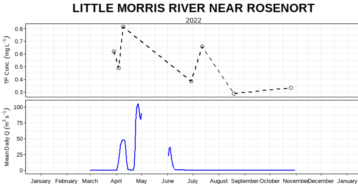
Figure 22: Mean daily discharge (m 3 s -1 ) and total phosphorus concentration (mg L -1 ) over the 2022 sampling season at Little Morris River near Rosenort (05OF024).
