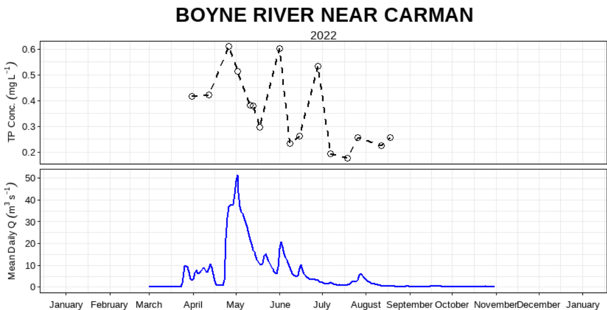
Figure 8: Mean daily discharge (m 3 s -1 ) and total phosphorus concentration (mg L -1 ) over the 2022 sampling season at Boyne River near Carman (05OF003).
