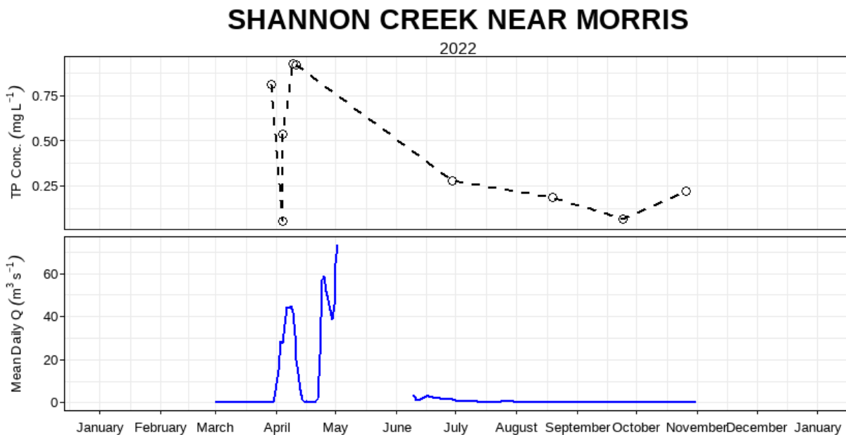
Figure 20: Mean daily discharge (m 3 s -1 ) and total phosphorus concentration (mg L -1 ) over the 2022 sampling season at Shannon Creek near Morris (05OF014).
