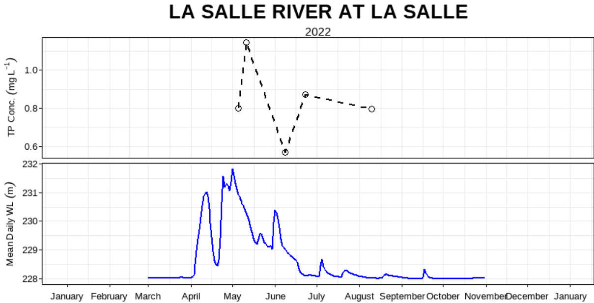
Figure 27: Mean daily water level (m) and total phosphorus concentration (mg L -1 ) at La Salle River at La Salle (05OG002).
