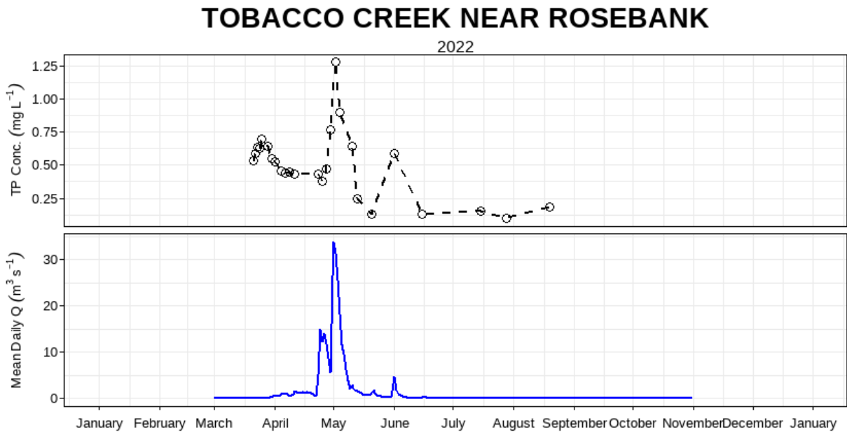
Figure 16: Mean daily discharge (m 3 s -1 ) and total phosphorus concentration (mg L -1 ) over the 2022 sampling season at Tobacco Creek near Rosebank (05OF018).
