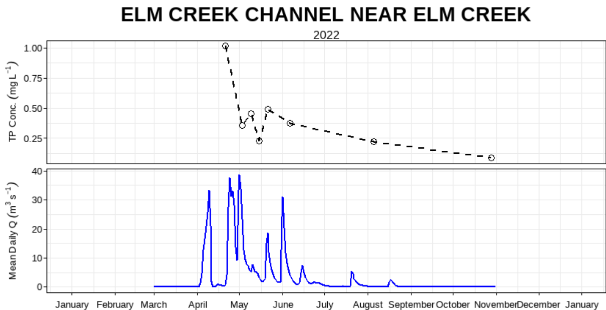
Figure 6: Mean daily discharge (m 3 s -1 ) and total phosphorus concentration (mg L -1 ) over the 2022 sampling season at Elm Creek Channel near Elm Creek (05OG005).
