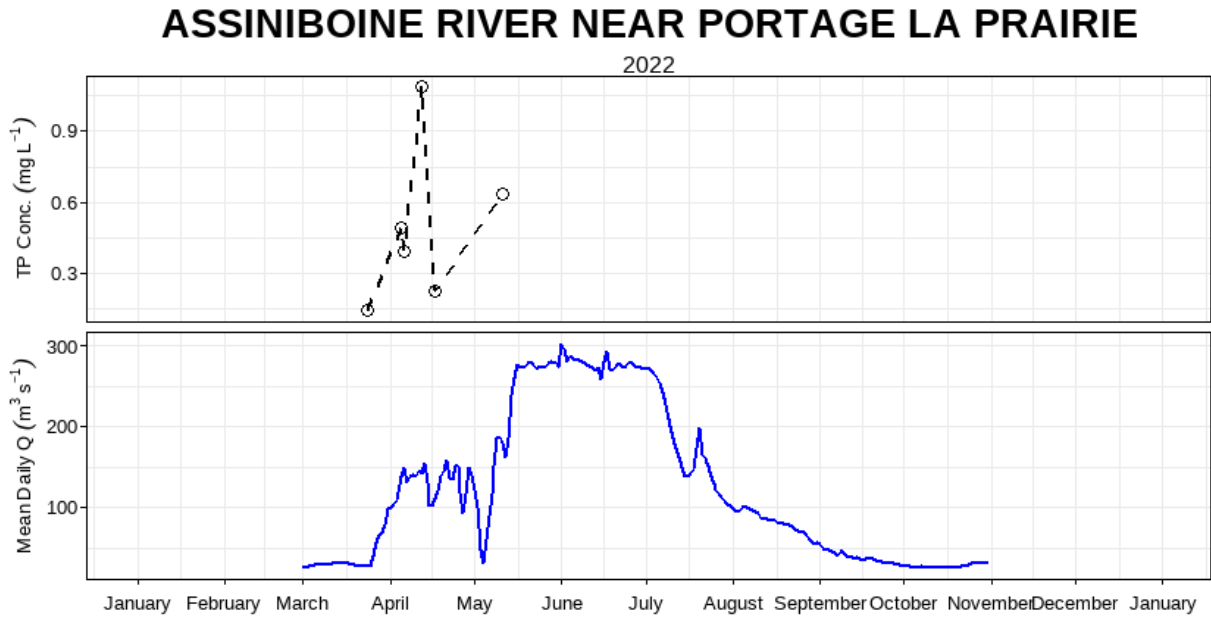
Figure 28: Mean daily discharge (m 3 s -1 ) and total phosphorus concentration (mg L -1 ) over the 2022 sampling season at Assiniboine River near Portage La Prairie (05MJ003).
