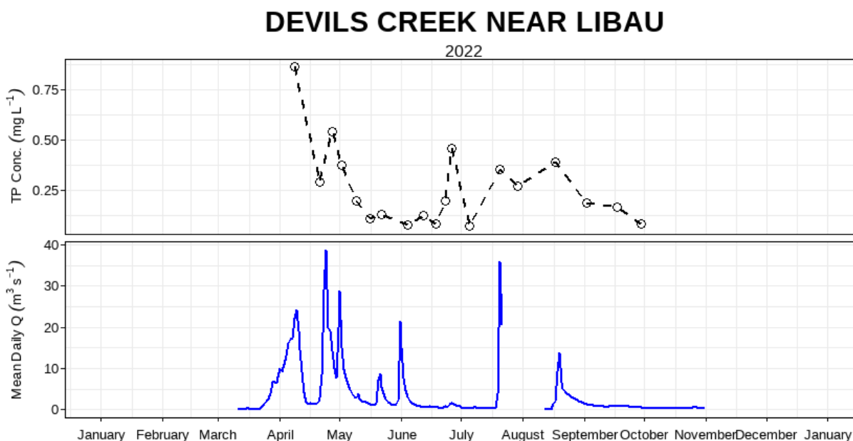
Figure 4: Mean daily discharge (m 3 s -1 ) and total phosphorus concentration (mg L -1 ) over the 2022 sampling season at Devil’s Creek near Libau (05OJ016).
