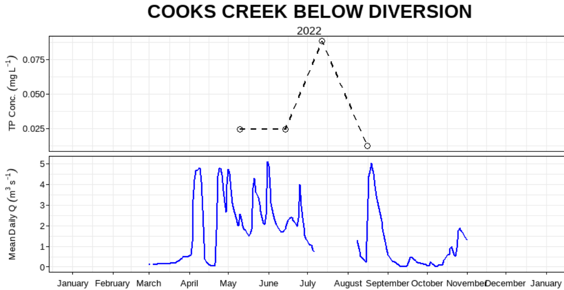
Figure 7: Mean daily discharge (m 3 s -1 ) and total phosphorus concentration (mg L -1 ) over the 2022 sampling season at Cooks Creek below Diversion (05OJ019).
