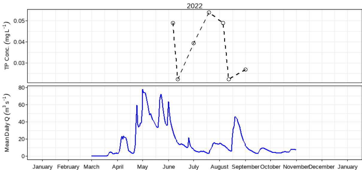
Figure 6: Mean daily discharge (m 3 s -1 ) and total phosphorus concentration (mg L -1 ) over the 2022 sampling season at Rolling River near Erickson (05MF008).
