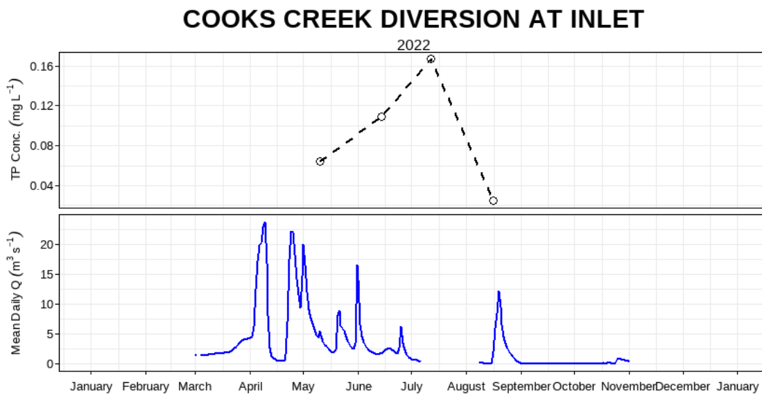
Figure 8: Mean daily discharge (m 3 s -1 ) and total phosphorus concentration (mg L -1 ) over the 2022 sampling season at Cooks Creek Diversion at Inlet (05OJ020).
