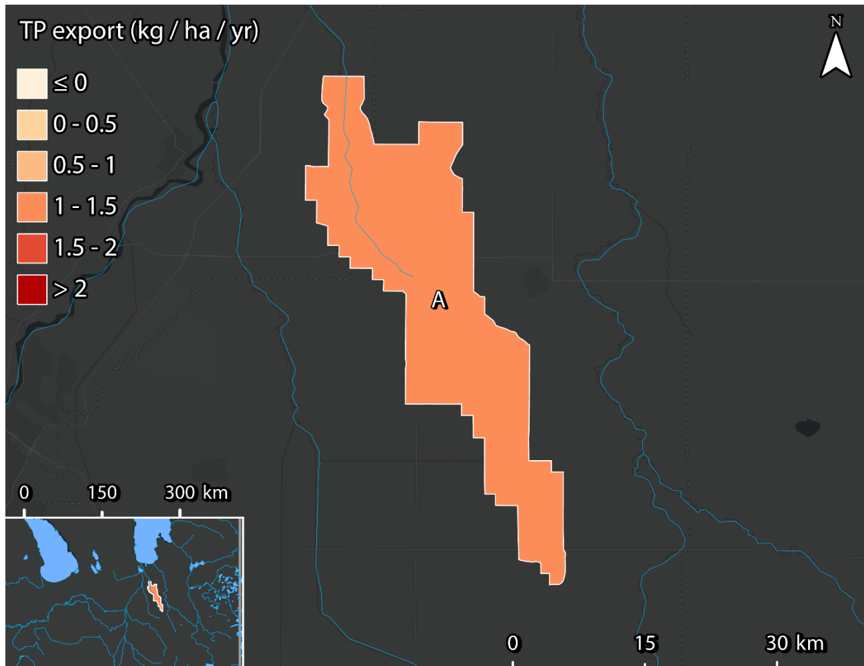
Figure 3: 2022 LWCBMN TP Export Hotspots in Northeast Red Watershed District. Letters correspond to sites listed in Table 2.
